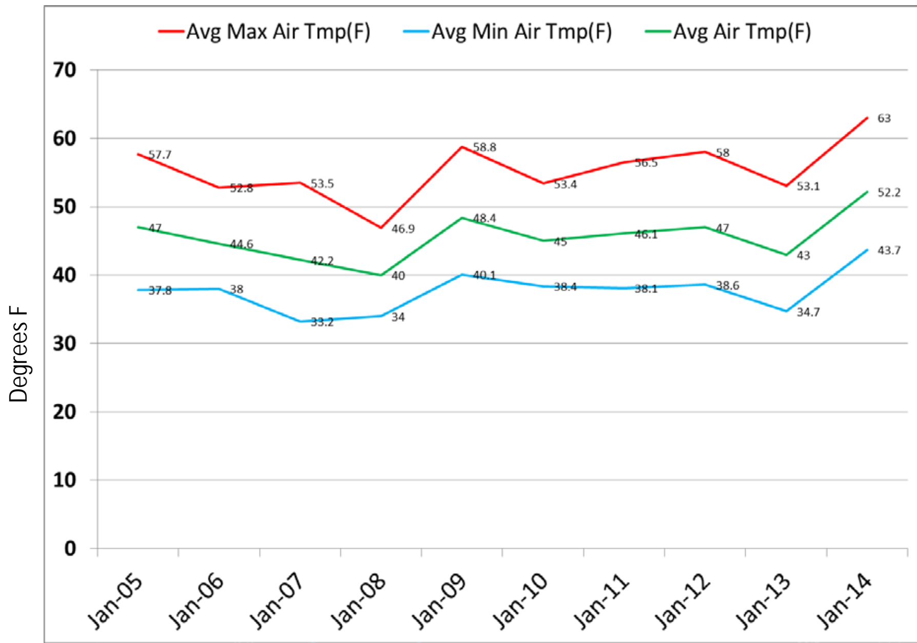
Average Max, Min, and Air Temperatures in January for the Past 10 Years (Camino CIMIS)
